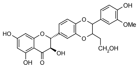
Isosilybin
