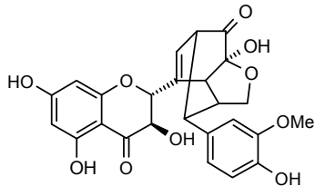
Silydianin
