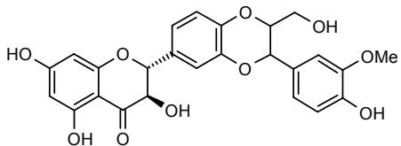
Silybin
